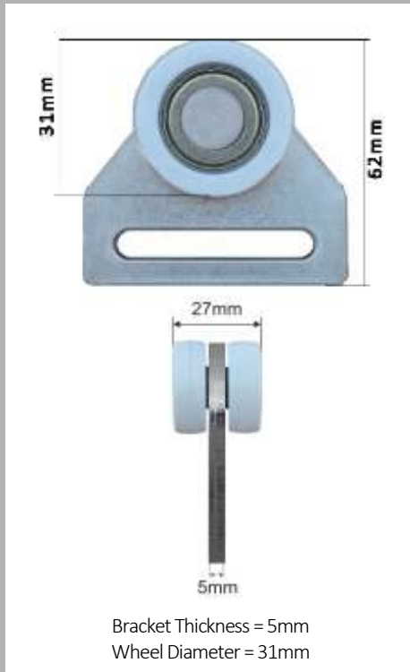
D31mm x W27mm = Part No: 113785
