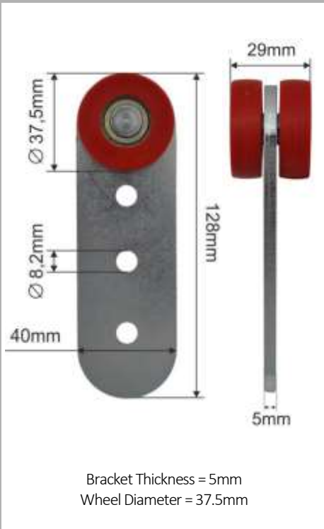
D37mm x W30mm = Part No: 113782
