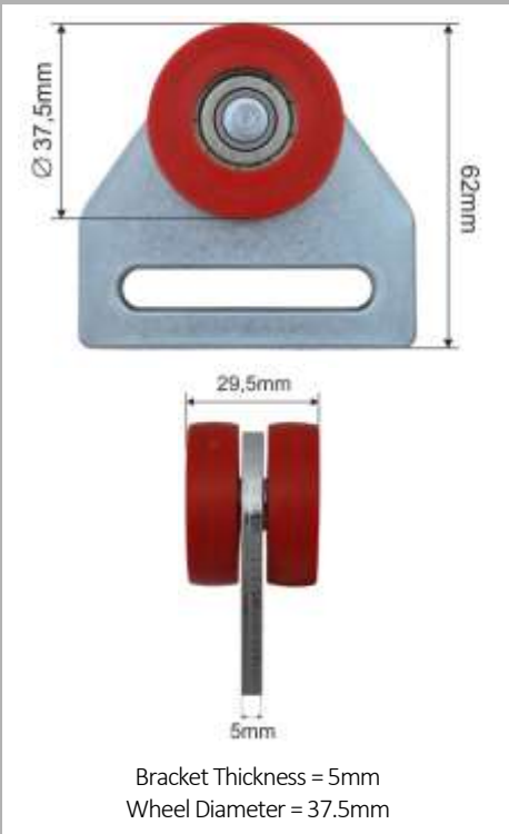
D37mm x W29mm = Part No: 113783
