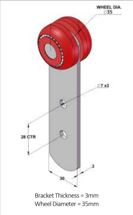
D35mm x W29mm = Part No: 113771 D35mm x W31mm = Part No: 113774
