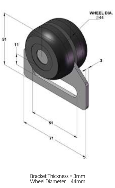
D44mm x W33mm = Part No: 113870
