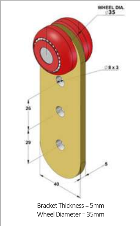
D35mm x W31mm = Part No: 113812
