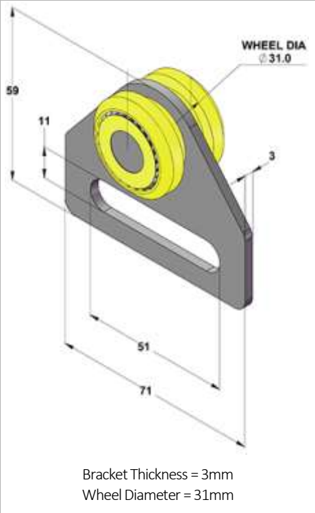
D31mm x W24mm = Part No: 113753 D31mm x W29mm = Part No: 113754
