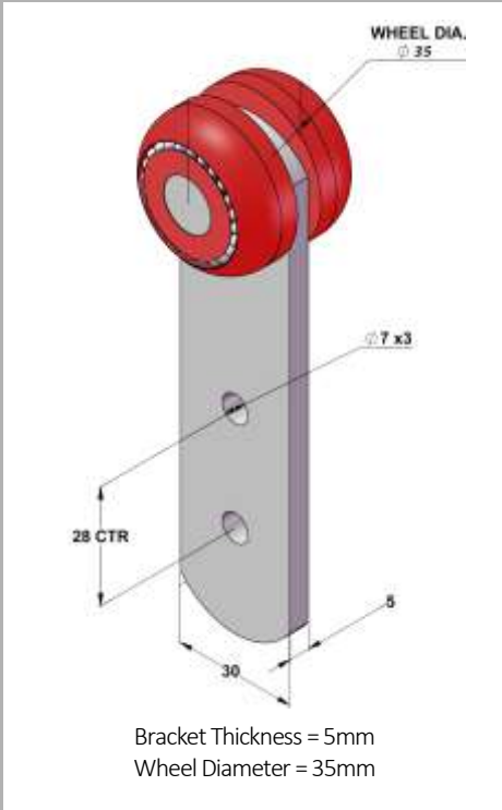
D35mm x W31mm = Part No: 113770
