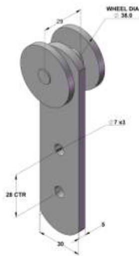
Bracket Thickness = 5mm Wheel Diameter = 38mm
