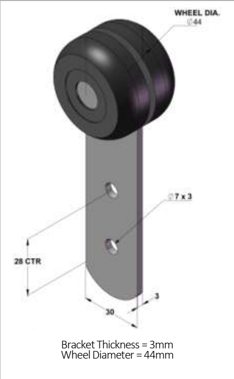
D44mm x W33mm = Part No: 113872
