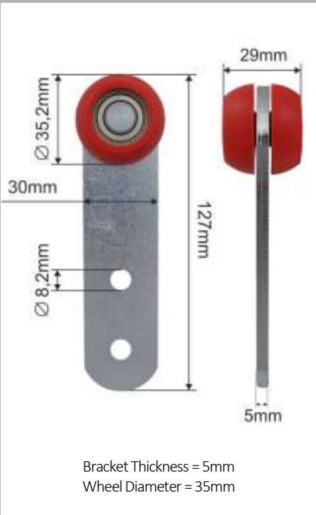
D35mm x W29mm = Part No: 113780
