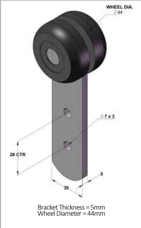
D44mm x W35mm = Part No: 113873
