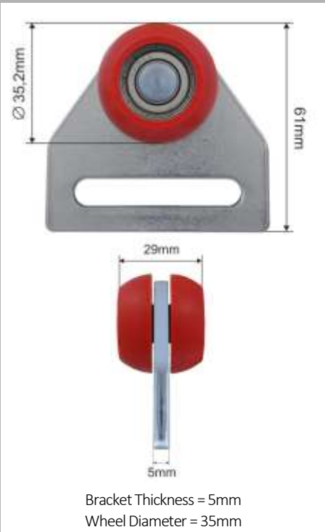
D35mm x W29mm = Part No: 113781
