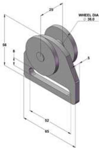
Bracket Thickness = 5mm Wheel Diameter = 38mm
