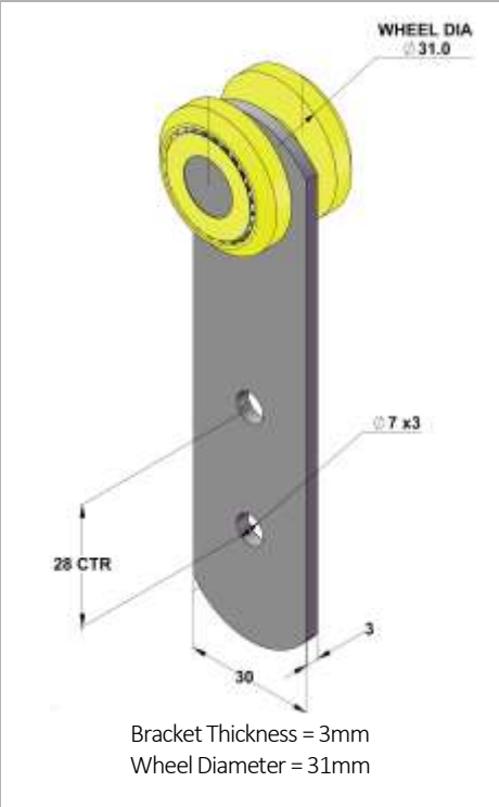
D31mm x W24mm = Part No: 113750 D31mm x W29mm = Part No: 113752
